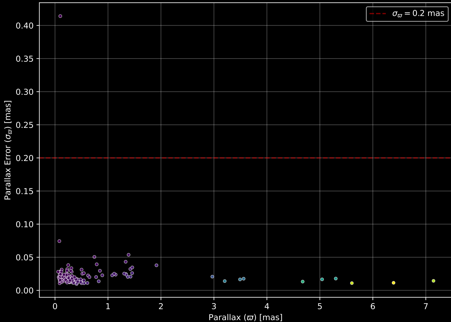
APOGEE DR17 Field: [235-06] Parallax Quality (n= 144)
