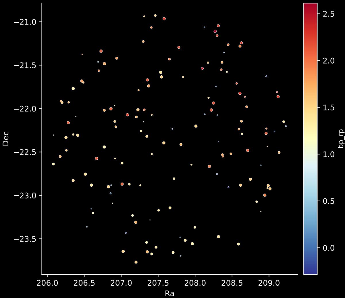
APOGEE DR17 Field: [235-06] Stars: 144
