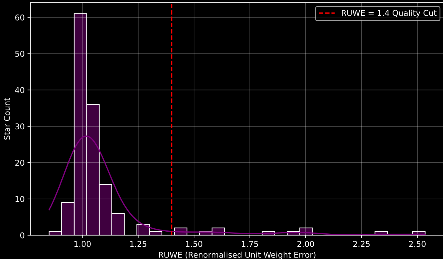
GAPOGEE DR17 Field [235-06] RUWE Distribution (n= 142)
