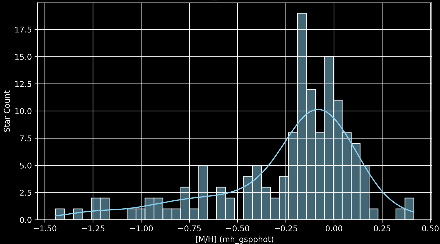
APOGEE DR17 Field: [235-06 [M/H] (mh_gspphot) (n= 143)
