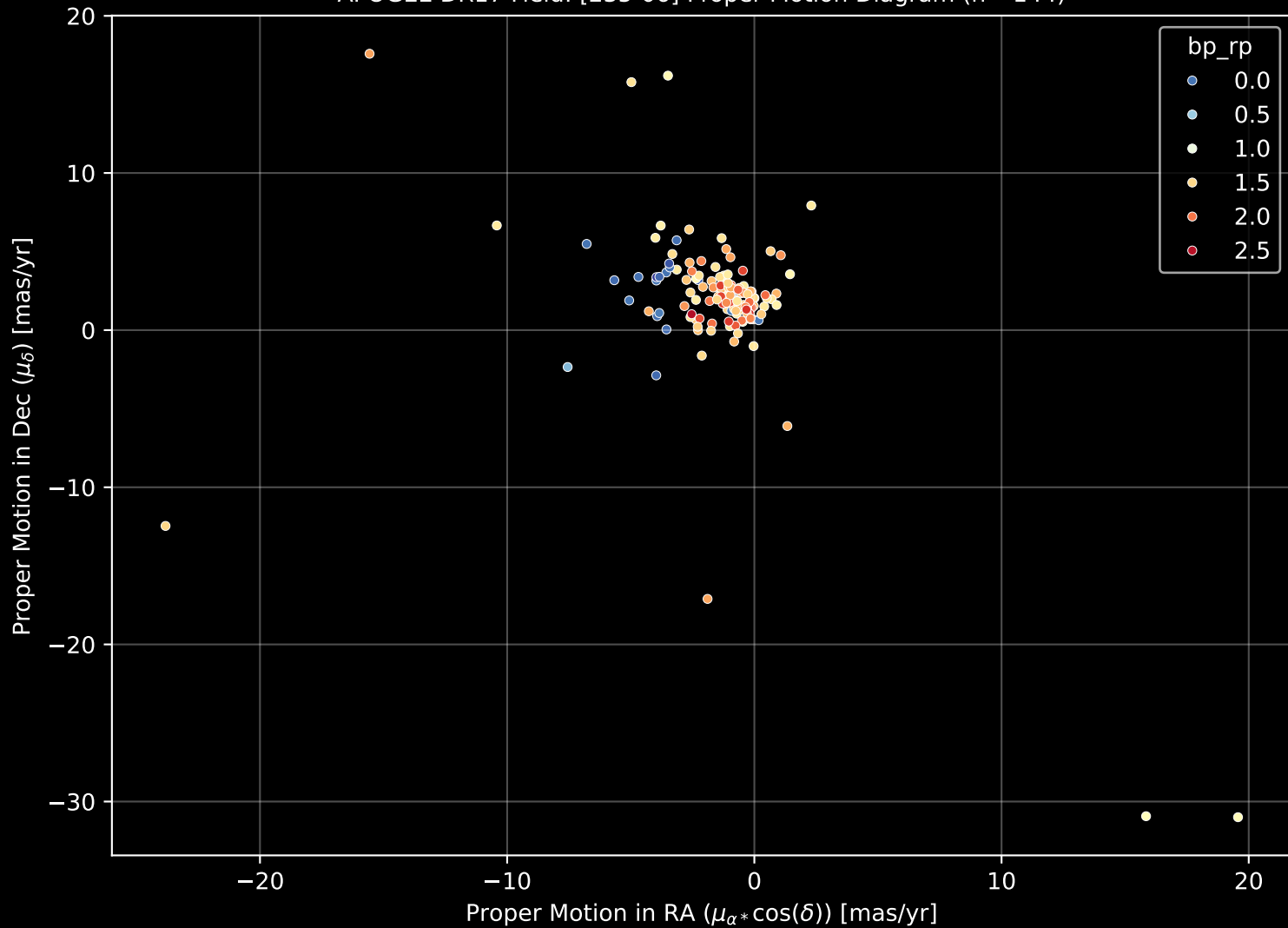
APOGEE DR17 Field: [235-06] Proper Motion Diagram (n= 144)
